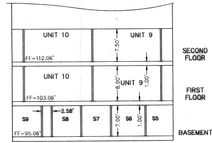
B TYPICAL FLOOR B VERTICAL VIEW WITH BASEMENT SCALE 1"=10'
