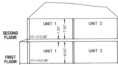
A TYPICAL FLOOR A VERTICAL VIEW WITHOUT BASEMENT SCALE 1"=10'
